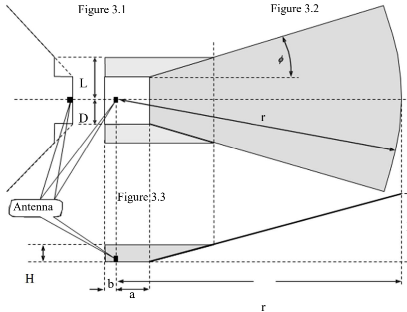
Shape to be applied for the directional facilities Figure 3.1 End elevation Figure 3.2 Plan elevation Figure 3.3 Side elevation
