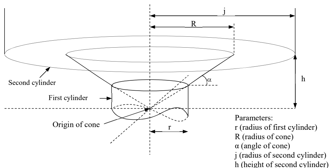
Figure 2.1: Omni - Directional BRA Shape (three dimensional representations)
